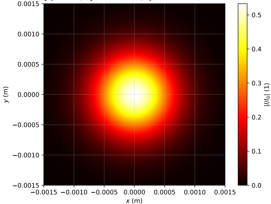
Intensity profile I(x, y, z = 2.468m)/I_0 , \text{Pin}=0.3\text{Pcr} , artificial time
